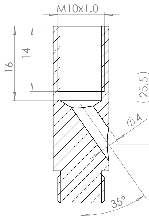
Section B-B
